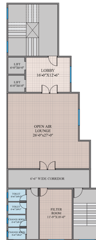
SEVENTH FLOOR PLAN
